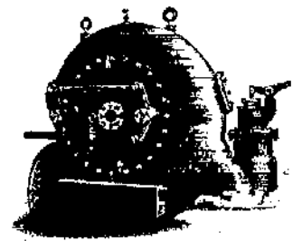
Single Horizontal Water Wheel, 360 h. p., under 100 ft. head, driving a 250 k. w. Alternator, Liskeard Light, Heat and Power Co. Bulletin 303.
