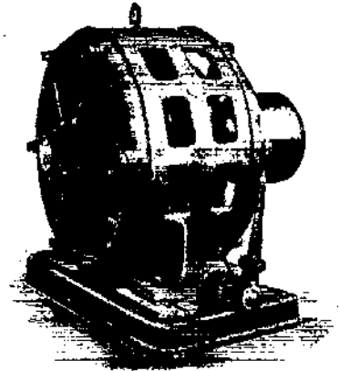
Single Horizontal Water Wheel, 360 h. p., under 100 ft. head, driving a 250 k. w. Alternator, Liskeard Light, Heat and Power Co. Bulletin 303.
