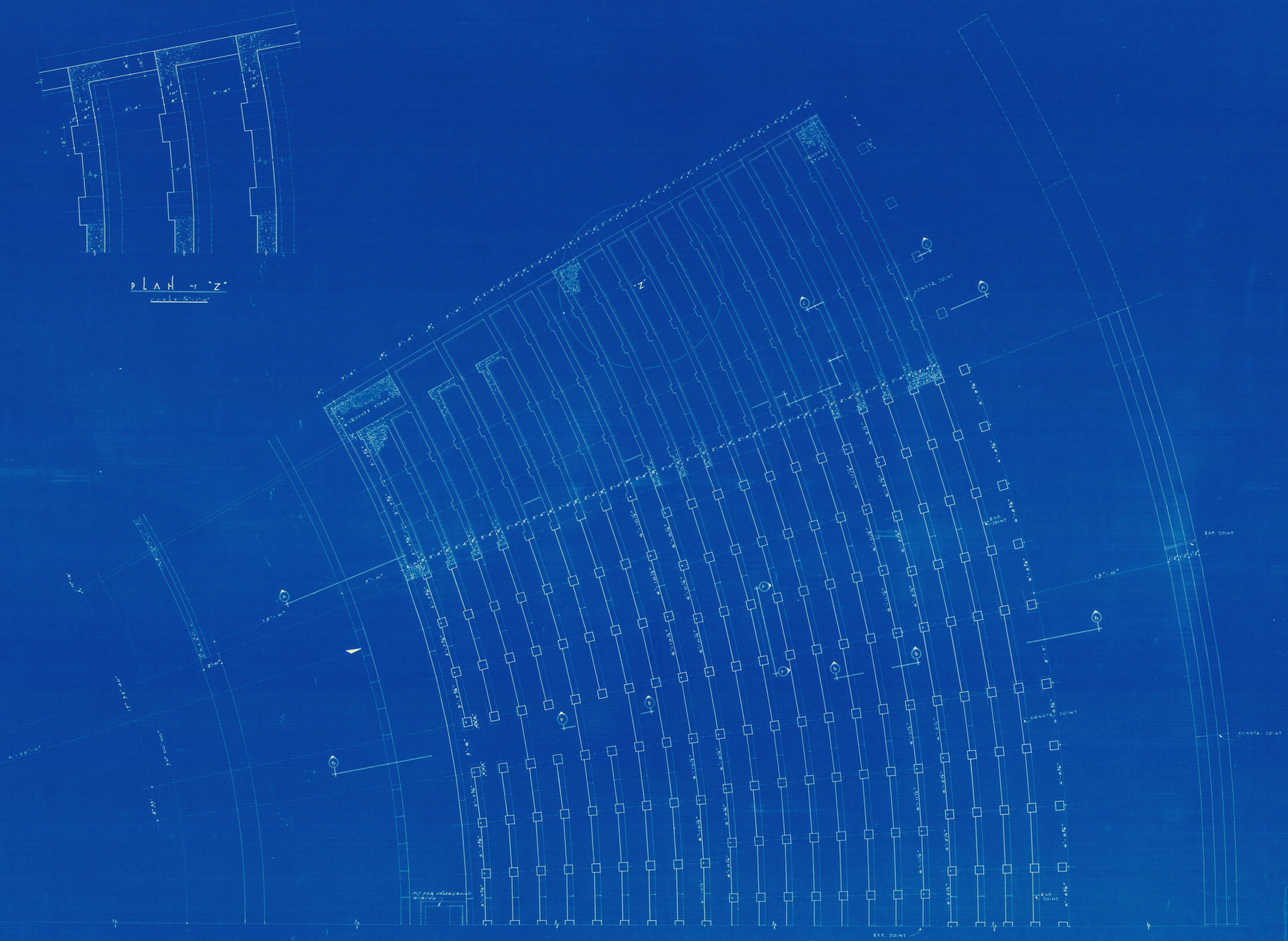
AUDITORIUM CONCRETE BASES FOR SEATS - SCALE 3/8"=1'-0"
