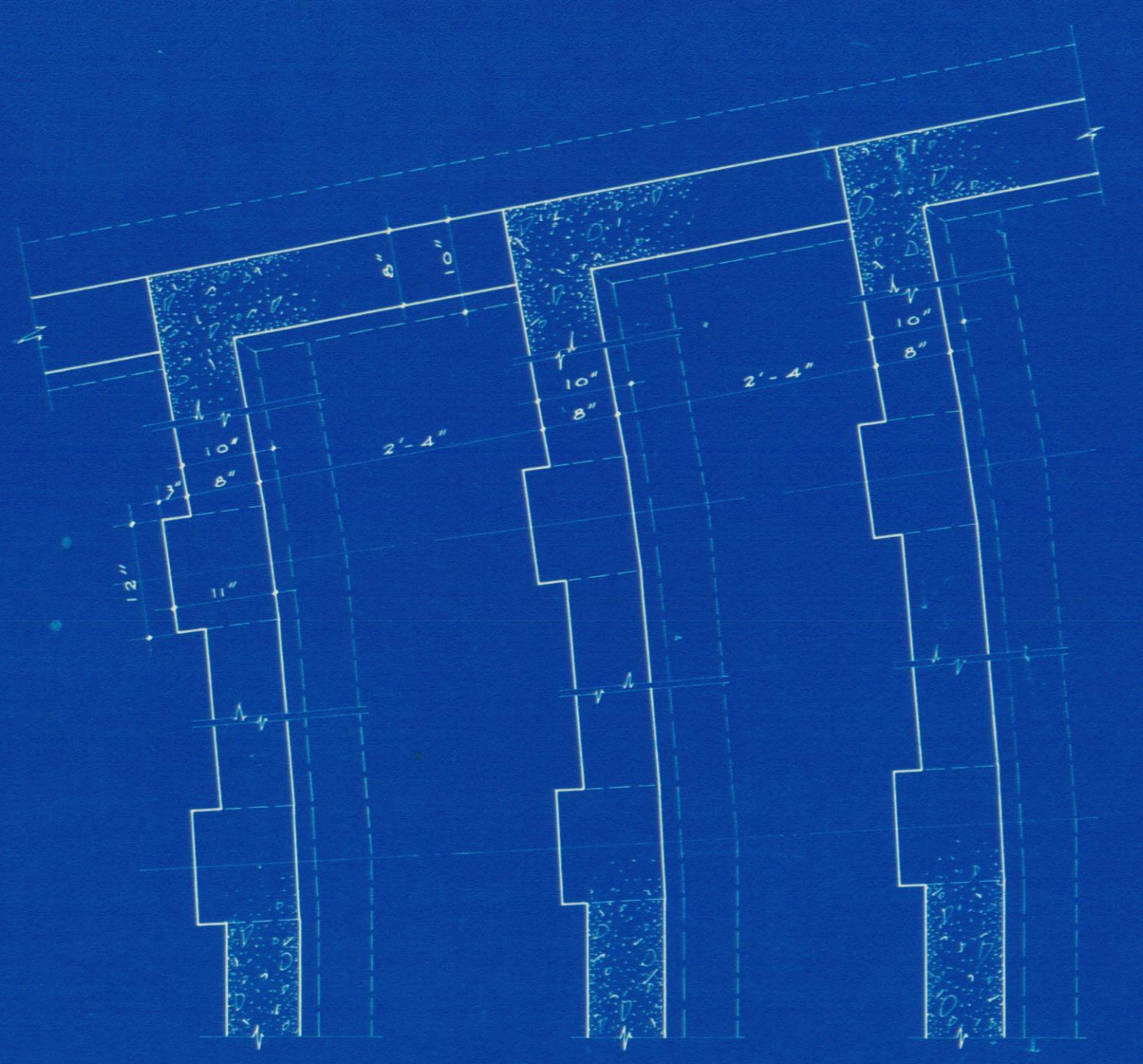
PLAN "Z" SCALE 3/8"=1'-0"
