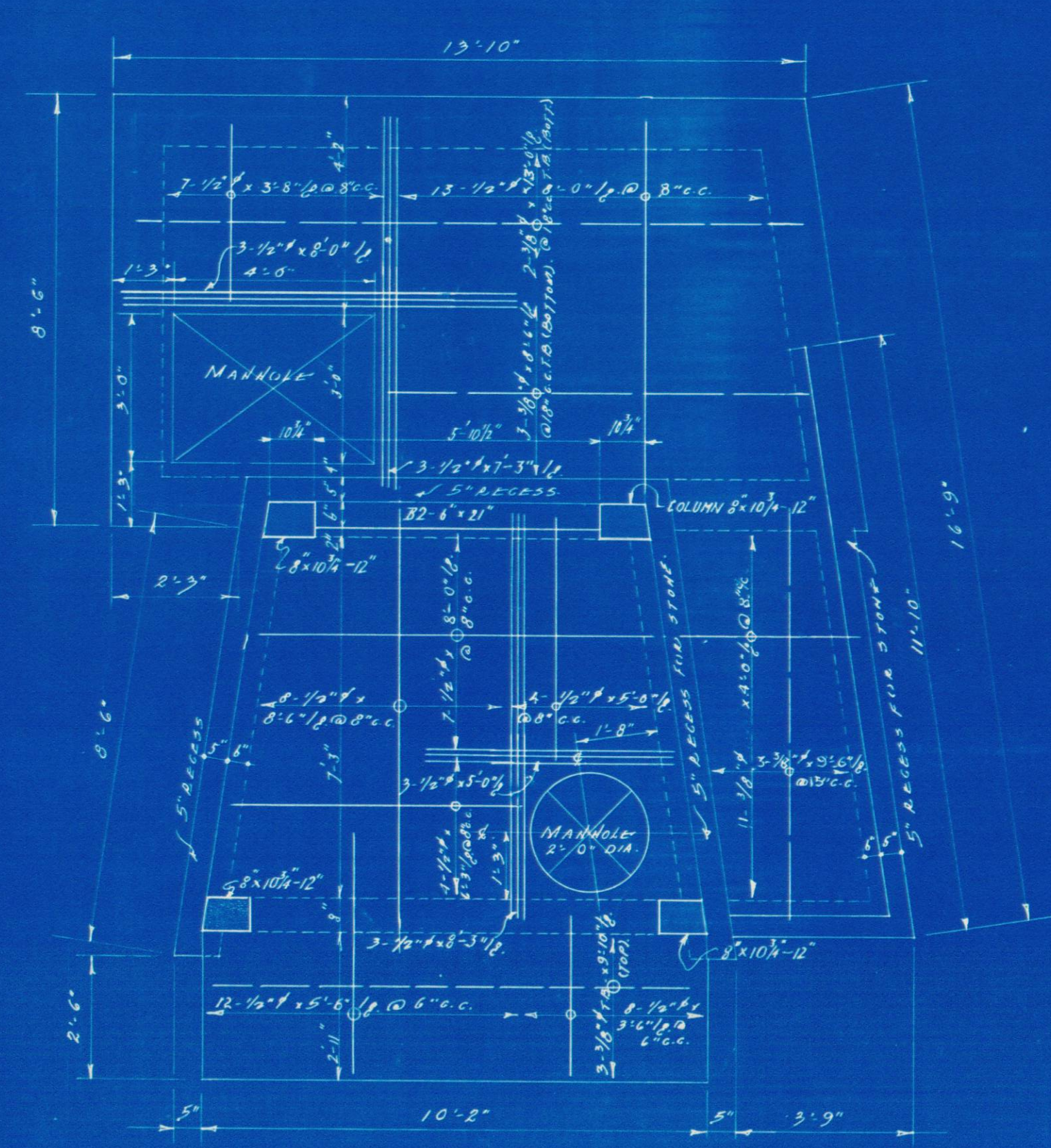
CONTROL ROOM & DIMMERS ROOM PLAN
