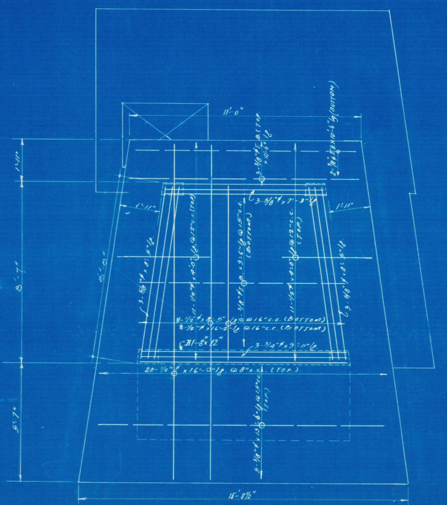
ROOF PLAN
