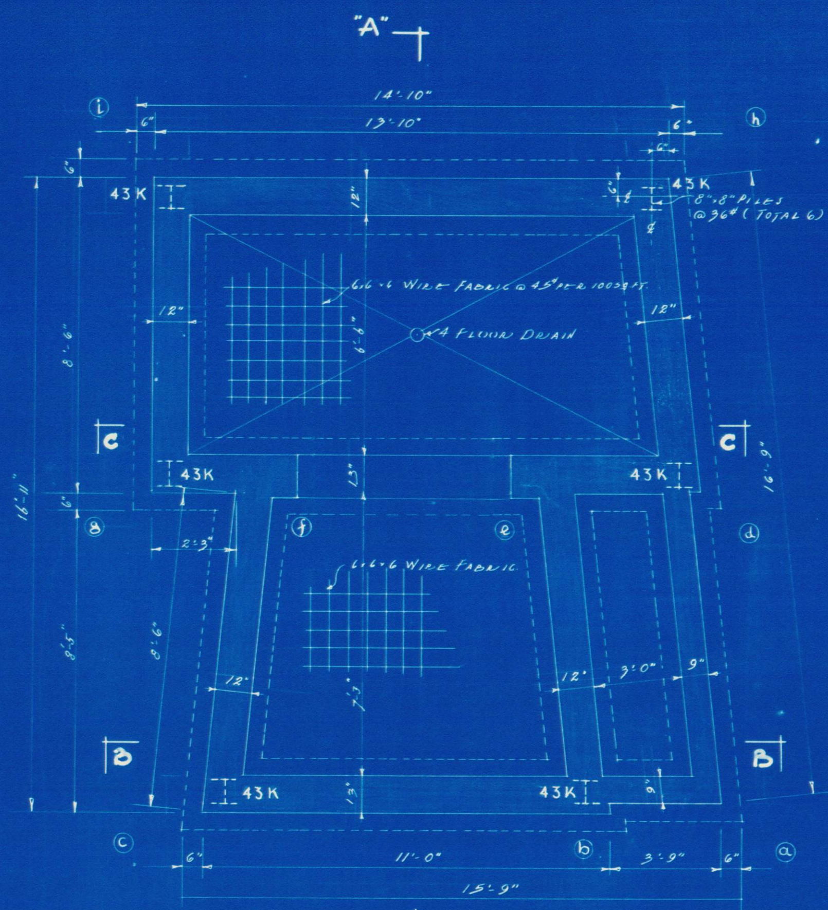
TRANSFORMER ROOM PLAN 1/4" = 1'-0"
