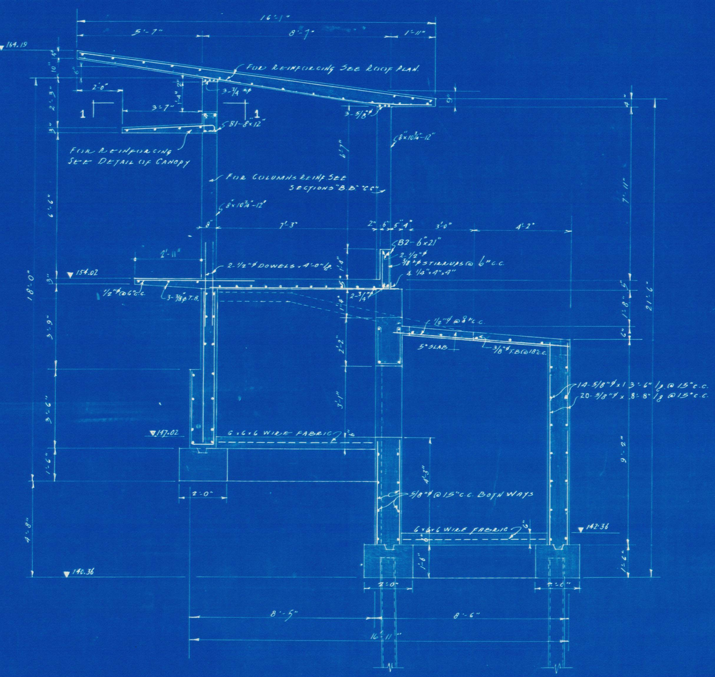
SECTION A-A 1/4" = 1'-0"
