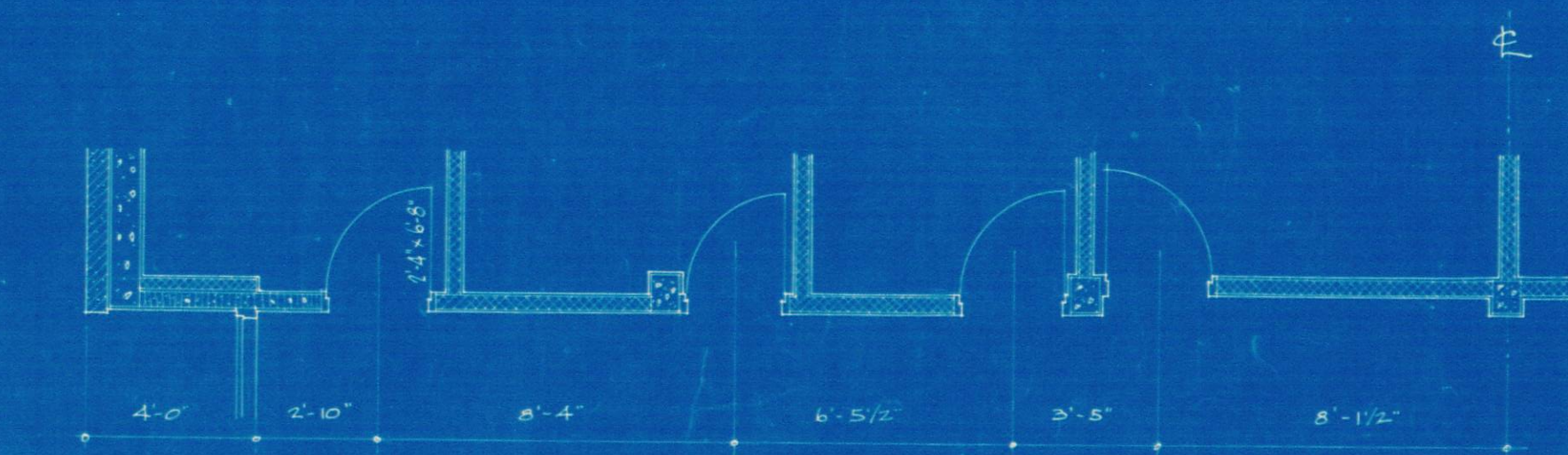
PASSAGE WALL SECTION THRU' DOORS 1/4" = 1'-0"
