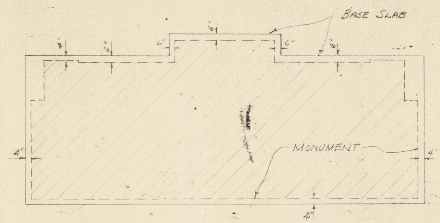
KEY PLAN SCALE 1/4" = 1'-0"
