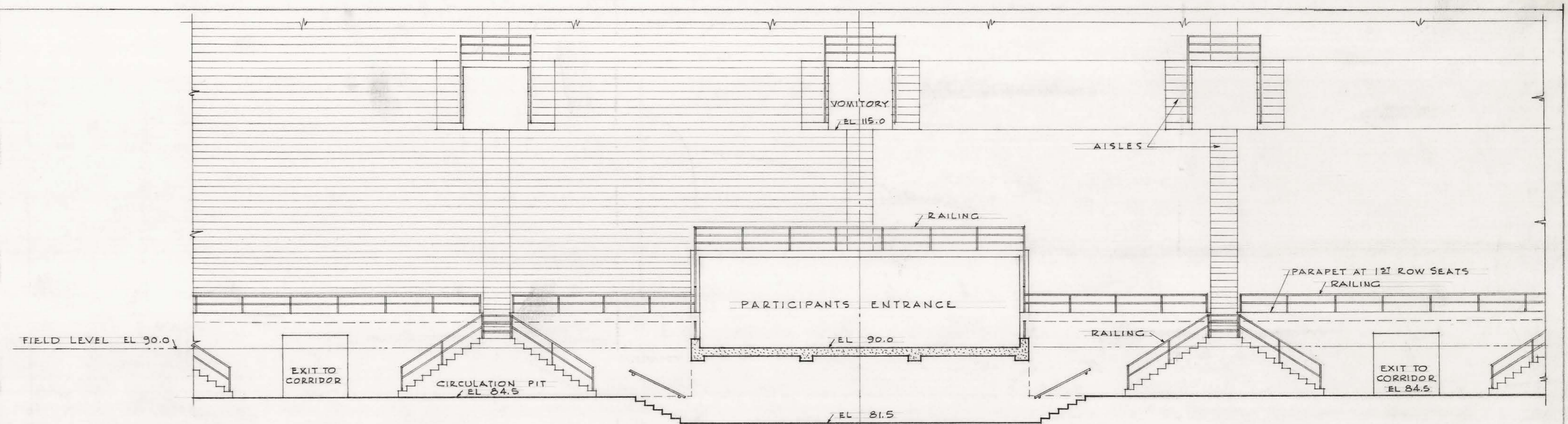
ELEVATION AT WEST ENTRANCE - FIELD SIDE DEVELOPED ON FACE OF PARAPET AT FIRST ROW OF SEATS HORIZONTAL LOCATION OF AISLES AND VOMITORIES IS DIAGRAMMATIC ONLY
